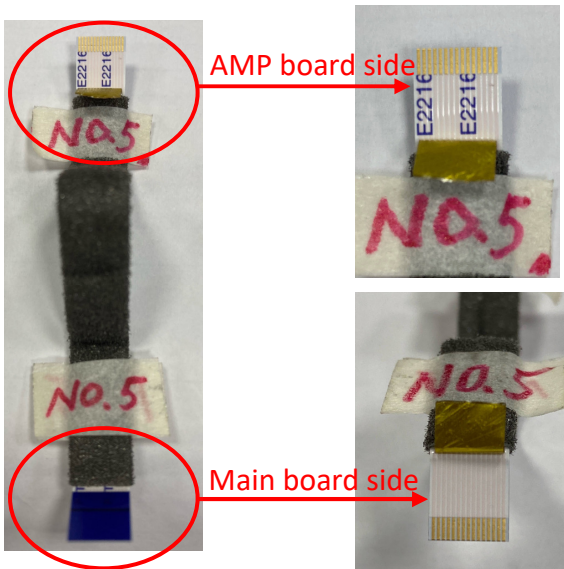
Combined thermal cycling test sample
